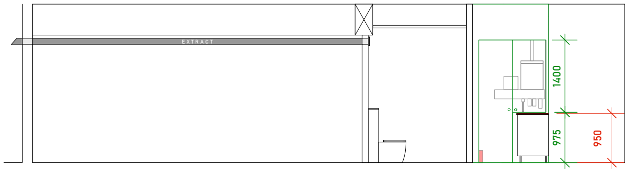
DRAY WALK GALLERY - SECTION 1:75 @ A4
